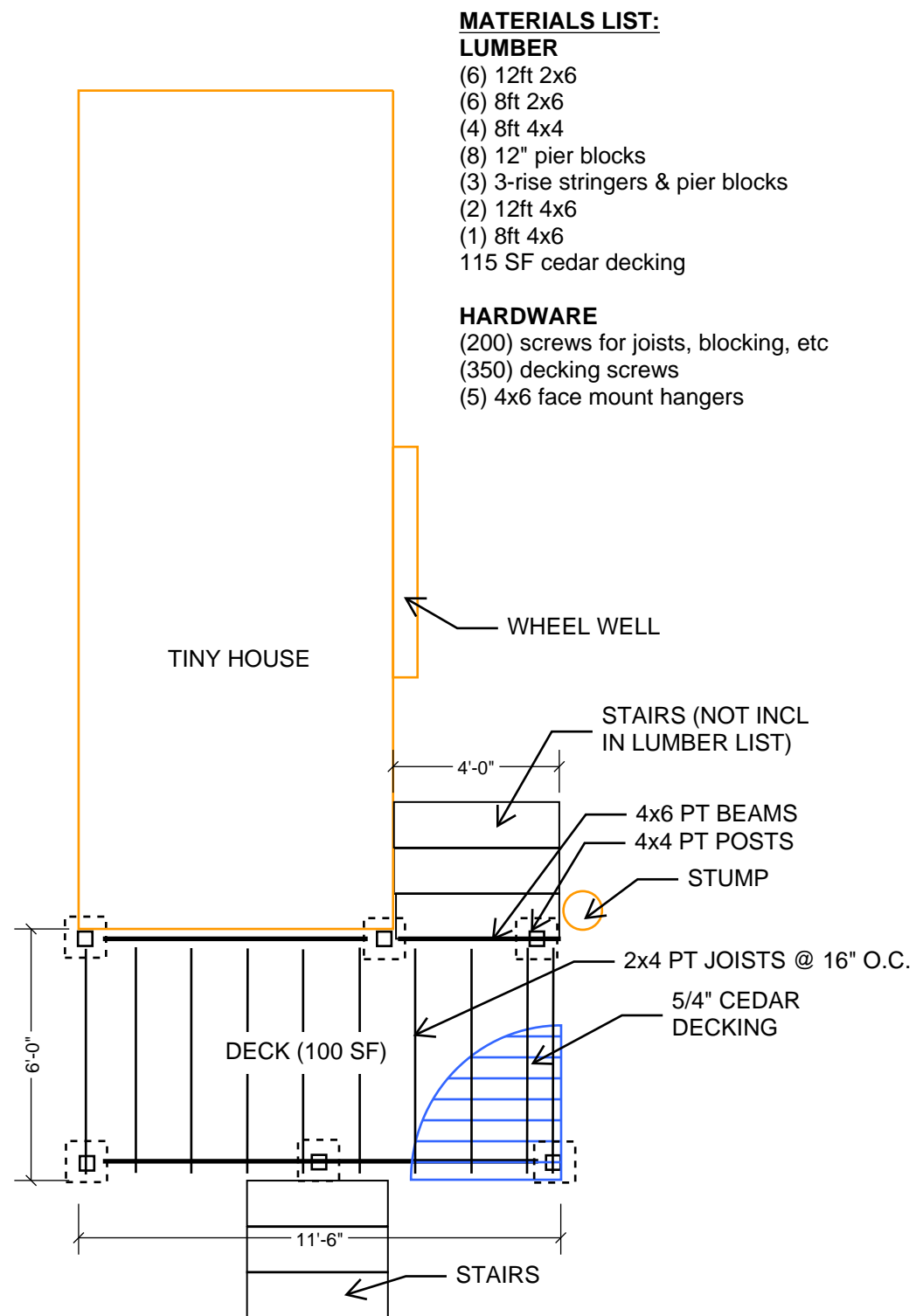
DECK FRAMING PLAN
